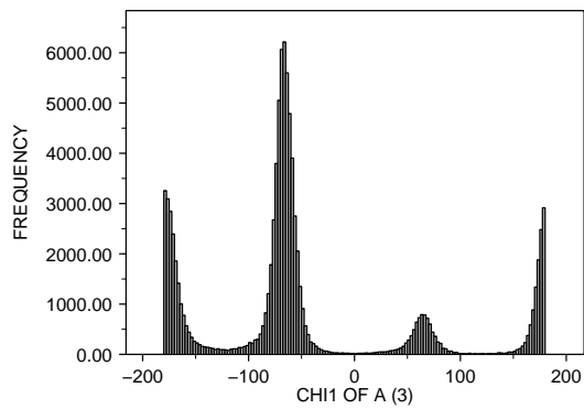
<2 : X-RAY RESOLUTION OF A (35) GLU : RESIDUE TYPE OF A (1) 94031.0 POINTS
