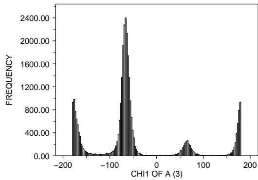
<2 : X-RAY RESOLUTION OF A (35) MET : RESIDUE TYPE OF A (1) 30504.0 POINTS
