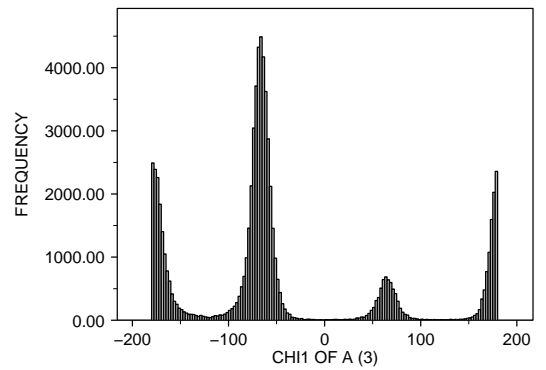
<2 : X-RAY RESOLUTION OF A (35) ARG : RESIDUE TYPE OF A (1) 71307.0 POINTS
