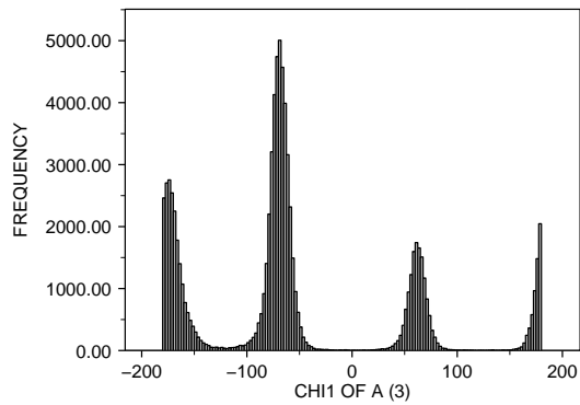
<2 : X-RAY RESOLUTION OF A (35) ASP : RESIDUE TYPE OF A (1) 82652.0 POINTS
