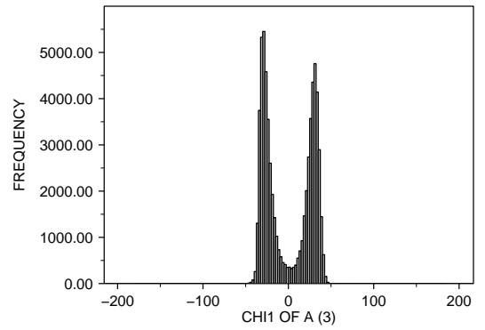
<2 : X-RAY RESOLUTION OF A (35) PRO : RESIDUE TYPE OF A (1) 65687.0 POINTS
