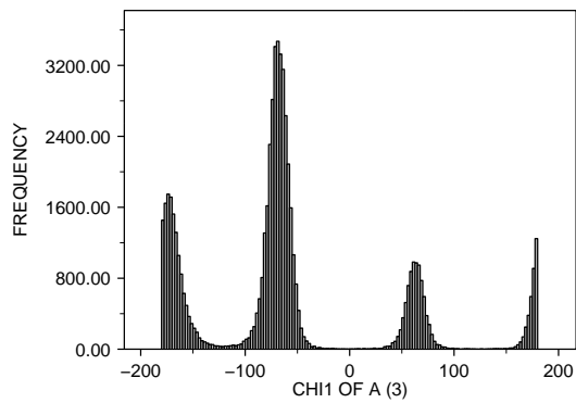
<2 : X-RAY RESOLUTION OF A (35) ASN : RESIDUE TYPE OF A (1) 59998.0 POINTS
