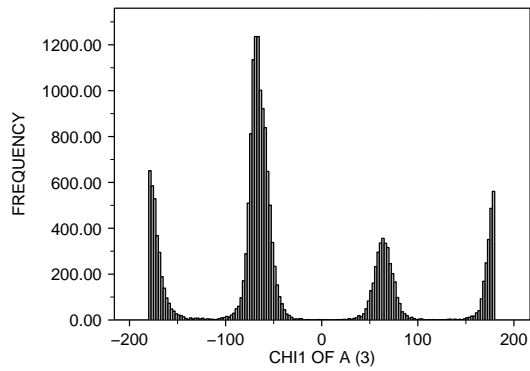
<2 : X-RAY RESOLUTION OF A (35) CYS : RESIDUE TYPE OF A (1) 19174.0 POINTS
