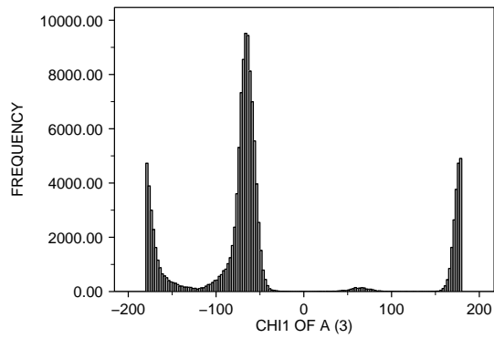
<2 : X-RAY RESOLUTION OF A (35) LEU : RESIDUE TYPE OF A (1) 129155.0 POINTS
