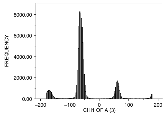
<2 : X-RAY RESOLUTION OF A (35) ILE : RESIDUE TYPE OF A (1) 80713.0 POINTS
