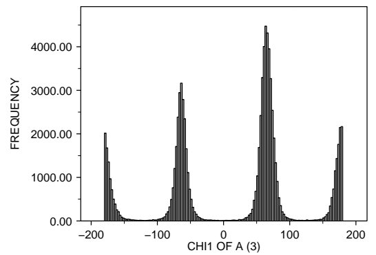
<2 : X-RAY RESOLUTION OF A (35) SER : RESIDUE TYPE OF A (1) 82844.0 POINTS
