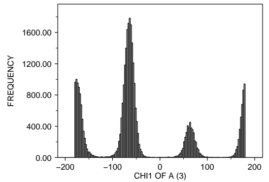
<2 : X-RAY RESOLUTION OF A (35) HIS : RESIDUE TYPE OF A (1) 33294.0 POINTS
