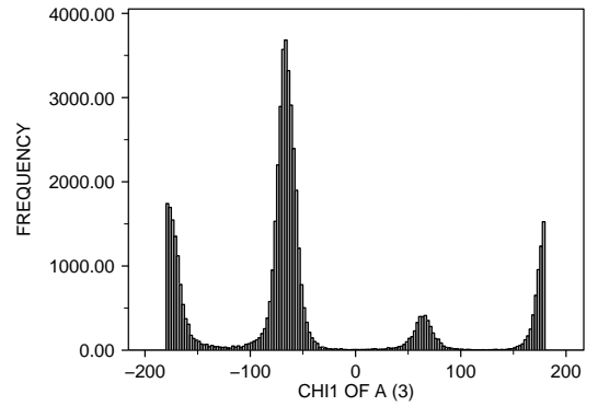
<2 : X-RAY RESOLUTION OF A (35) GLN : RESIDUE TYPE OF A (1) 51404.0 POINTS
