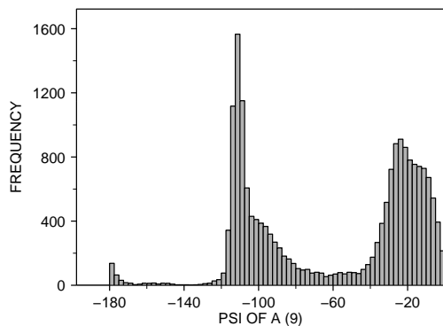
<2 : X-RAY RESOLUTION OF A (35) CYS : RESIDUE TYPE OF A (1) 19093.0 POINTS
