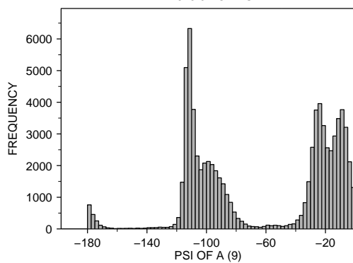
<2 : X-RAY RESOLUTION OF A (35) THR : RESIDUE TYPE OF A (1) 77625.0 POINTS
