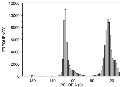
<2 : X-RAY RESOLUTION OF A (35) VAL : RESIDUE TYPE OF A (1) 102793.0 POINTS
