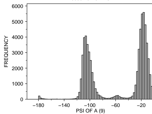
<2 : X-RAY RESOLUTION OF A (35) PRO : RESIDUE TYPE OF A (1) 65397.0 POINTS
