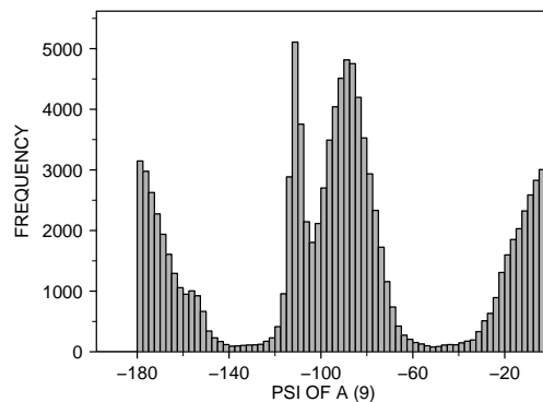
<2 : X-RAY RESOLUTION OF A (35) GLY : RESIDUE TYPE OF A (1) 107770.0 POINTS
