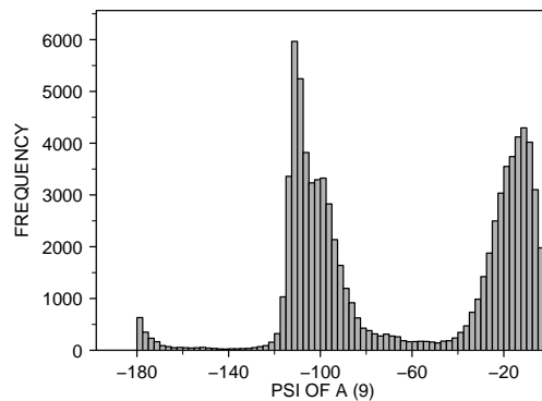
<2 : X-RAY RESOLUTION OF A (35) SER : RESIDUE TYPE OF A (1) 82728.0 POINTS
