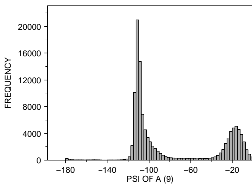
<2 : X-RAY RESOLUTION OF A (35) ALA : RESIDUE TYPE OF A (1) 118089.0 POINTS
