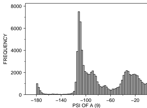
<2 : X-RAY RESOLUTION OF A (35) ASP : RESIDUE TYPE OF A (1) 82901.0 POINTS
