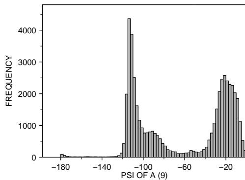
<2 : X-RAY RESOLUTION OF A (35) TYR : RESIDUE TYPE OF A (1) 50006.0 POINTS
