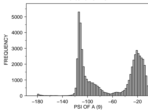
<2 : X-RAY RESOLUTION OF A (35) PHE : RESIDUE TYPE OF A (1) 57092.0 POINTS
