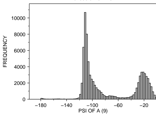
<2 : X-RAY RESOLUTION OF A (35) LYS : RESIDUE TYPE OF A (1) 81306.0 POINTS
