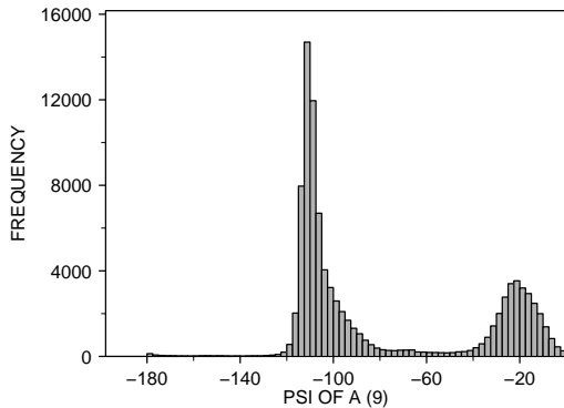
<2 : X-RAY RESOLUTION OF A (35) GLU : RESIDUE TYPE OF A (1) 95009.0 POINTS
