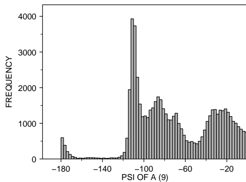
<2 : X-RAY RESOLUTION OF A (35) ASN : RESIDUE TYPE OF A (1) 60020.0 POINTS
