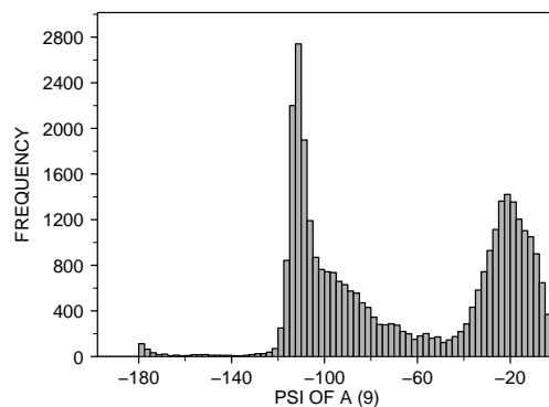
<2 : X-RAY RESOLUTION OF A (35) HIS : RESIDUE TYPE OF A (1) 33262.0 POINTS
