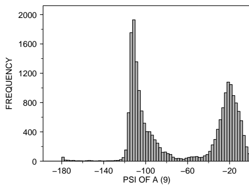
<2 : X-RAY RESOLUTION OF A (35) TRP : RESIDUE TYPE OF A (1) 20383.0 POINTS
