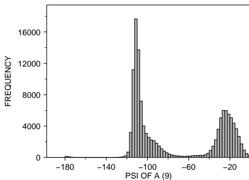
<2 : X-RAY RESOLUTION OF A (35) LEU : RESIDUE TYPE OF A (1) 128805.0 POINTS
