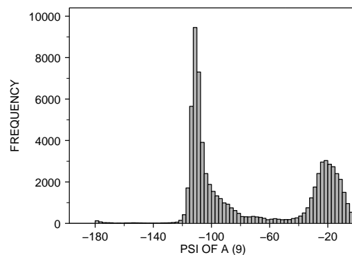
<2 : X-RAY RESOLUTION OF A (35) ARG : RESIDUE TYPE OF A (1) 71787.0 POINTS
