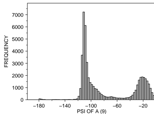
<2 : X-RAY RESOLUTION OF A (35) GLN : RESIDUE TYPE OF A (1) 51638.0 POINTS
