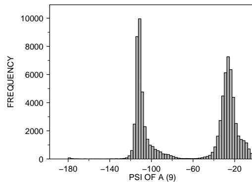
<2 : X-RAY RESOLUTION OF A (35) ILE : RESIDUE TYPE OF A (1) 80599.0 POINTS
