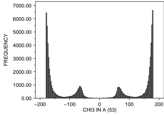
<2 : X-RAY RESOLUTION OF A (35) LYS : RESIDUE TYPE OF A (1) 78942.0 POINTS
