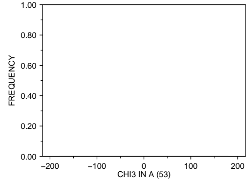
<2 : X-RAY RESOLUTION OF A (35) SER : RESIDUE TYPE OF A (1) 0.0 POINTS
