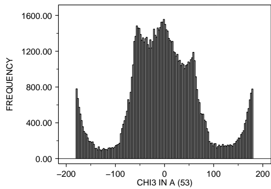
<2 : X-RAY RESOLUTION OF A (35) GLU : RESIDUE TYPE OF A (1) 93466.0 POINTS
