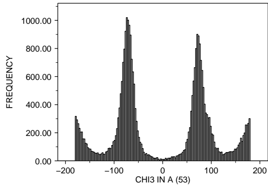
<2 : X-RAY RESOLUTION OF A (35) MET : RESIDUE TYPE OF A (1) 30482.0 POINTS
