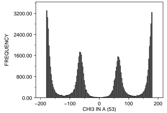
<2 : X-RAY RESOLUTION OF A (35) ARG : RESIDUE TYPE OF A (1) 70968.0 POINTS
