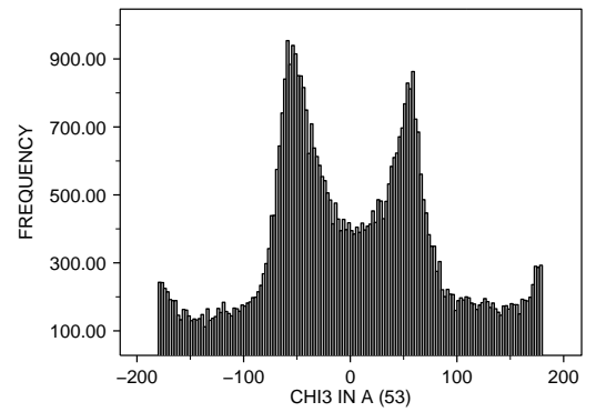
<2 : X-RAY RESOLUTION OF A (35) GLN : RESIDUE TYPE OF A (1) 51239.0 POINTS
