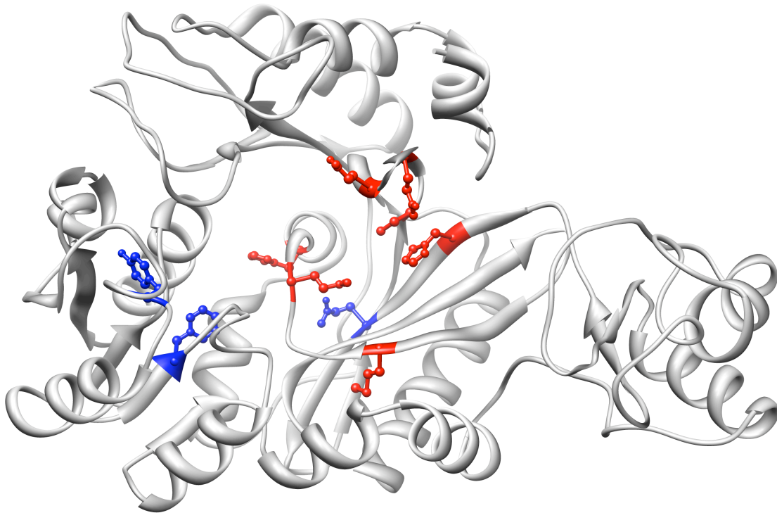
Figure 2. Model of Helicobacter pylori biotin carboxylase based on template 1dv1. TSVMMod predicts a C ^{\alpha} RMSD of 3.5 Å. The top ten functional residues predicted by INTREPID are highlighted: seven that are also known from the literature to be involved in catalytic function are colored red, and three representing potential novel predictions are colored blue. These ten residues are, in descending order of INTREPID importance score: C243 (red), H222 (red), H312 (red), F93 (blue), M304 (red), Y74 (blue), Q226 (blue), Q246 (red), Q250 (red), and Q309 (red). UCSF Chimera was used to load the model from ModBase and produce this figure.
