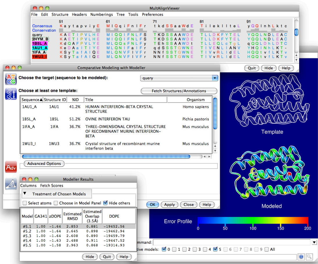
Figure 1: The Chimera – Modeller interface. The sequence alignment is displayed in Chimera's Multalign Viewer tool (top). In the dialog for running Modeller (middle left), one of the sequences in the alignment is designated as the target, and at least one structure (associated with another sequence in the alignment) is designated as the template. Structure information is shown to help guide the choice of template. After the run, the resulting models are listed along with various model scores from Modeller in a table (bottom left) and their structures are loaded into Chimera. In this example, the main Chimera window (right) shows the template as an outline and one of the model structures as a ribbon colored by error profile.
