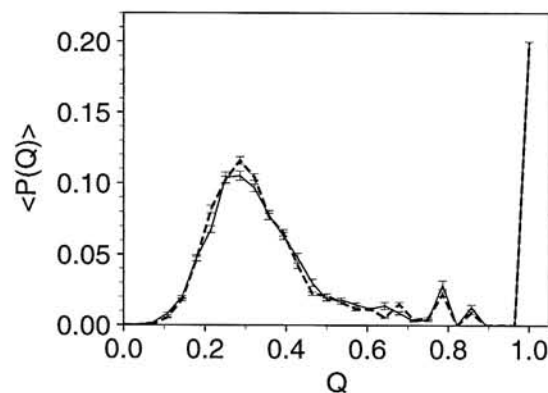
Figure 12. \langle P_T^{csa}(Q) \rangle for strongly folding and non-folding sequences. The shape of \langle P_T^{csa}(Q) \rangle for the folding sequences remains the same when only 15 sequences with foldicity of at least 0.80 are used in the average. Continuous and broken lines are used for the folding and non-folding sequences, respectively. The error bars indicate the standard error of the mean.
