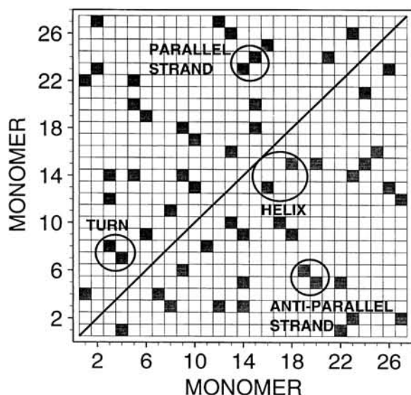
Figure 9. Definition of secondary structure segments (Chan & Dill, 1991). A contact map for sequence 43 is shown. A dark stippled square indicates a contact between the 2 corresponding monomers. The minimal length of a helix, parallel strand and anti-parallel strand is 2 contacts. A turn always has 2 contacts. Anti-parallel strand and helix contacts can include turn contacts.
