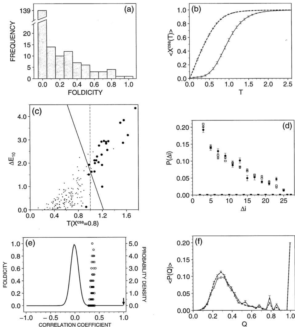
Figure 16. Associations for the multiple occupancy Monte Carlo algorithm. This Figure repeats the plots in Figs 4 (a), 6 (b), 7 (c), 8 (d), 10 (e) and 12 (f) with the data from the multiple occupancy Monte Carlo algorithm. See the legends to the original Figures for explanation. There are 25 strongly folding and 139 non-folding sequences for this algorithm.
