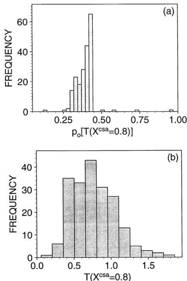
Figure 3. Determination of folding temperature. (a) Distribution of Boltzmann probabilities of the native structure for the 200 random sequences at T(X^{csa} = 0.8) . The Boltzmann probabilities were calculated using an ensemble of compact self-avoiding chains only. (b) Distribution of T(X^{csa} = 0.8) for the 200 random sequences in the database.
