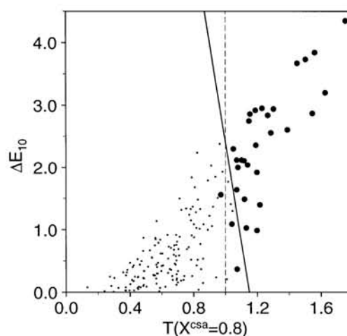
Figure 7. Discrimination between strongly folding and non-folding sequences on the basis of the energy gap, \Delta E_{10} , and T_x . Strongly folding sequences, filled circles; non-folding sequences, dots. The weakly folding sequences (not shown) are concentrated around the boundary between the strongly folding and non-folding sequences. They were omitted from the plot in order to obtain better contrast between folding and non-folding sequences. The continuous line separates the 2 groups of sequences by minimizing the number of the folding and non-folding sequences in the non-folding and folding parts of the plot, respectively. The broken line indicates the critical temperature T_c for the ensemble of compact self-avoiding chains estimated from Fig. 17(b) using eqn (5).
