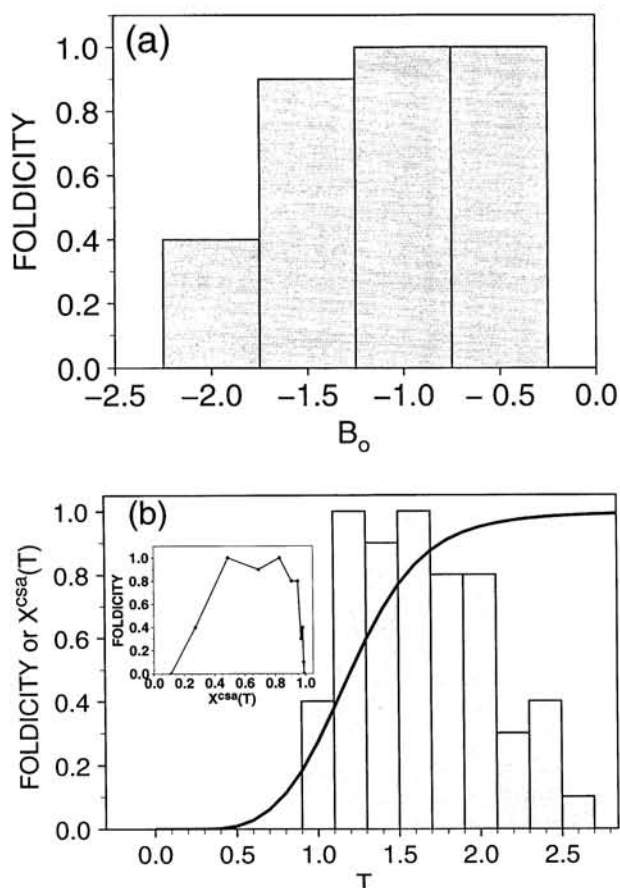
Figure 2. Optimal folding conditions for the trial folding sequence 2. Foldicity is determined from 10 independent Monte Carlo folding simulations. (a) The dependence of foldicity on the collapse parameter B_0 at T = 1.0 . (b) The histogram shows the dependence of foldicity on temperature T at B_0 = -2.0 . The curve is X^{csa}(T) on the same scale. The inset shows the dependence of foldicity on X^{csa}(T) .
