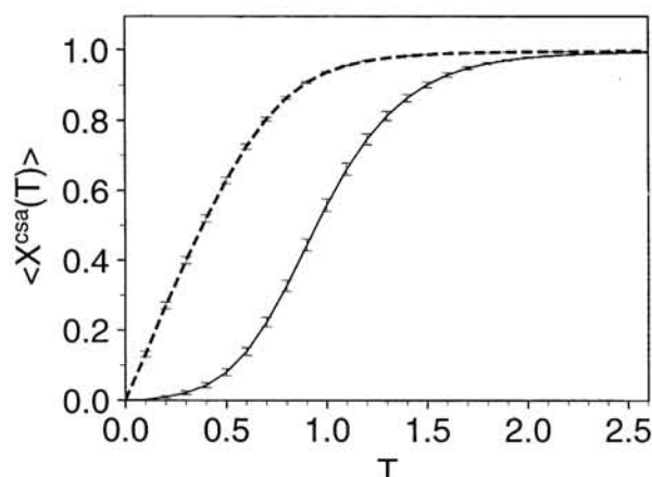
Figure 6. \langle X^{\text{csa}}(T) \rangle for strongly folding (continuous line) and non-folding (broken line) sequences at \tau = 1 . The error bars show the standard error of the mean.
